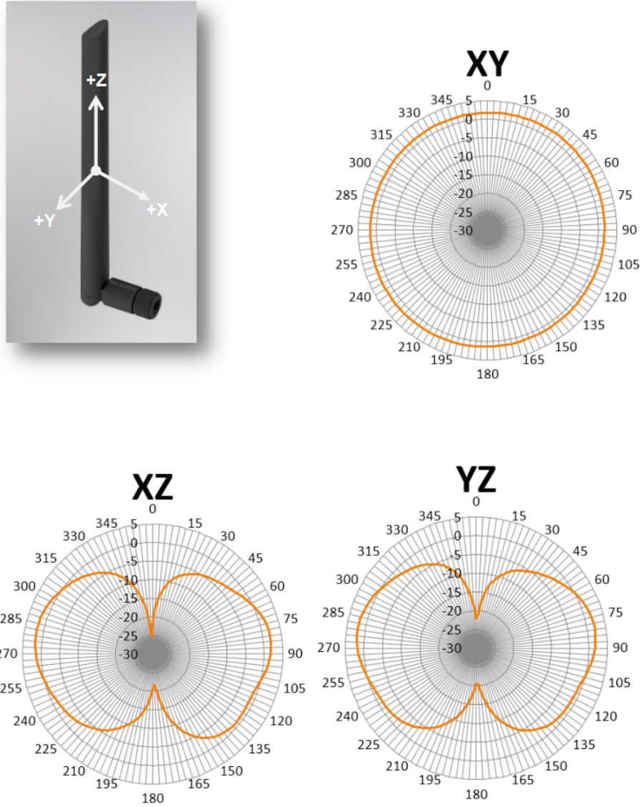
Figure 3: Radiation Patterns
