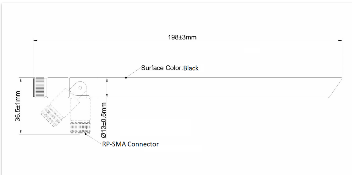
Figure 4: Mechanical Specifications
