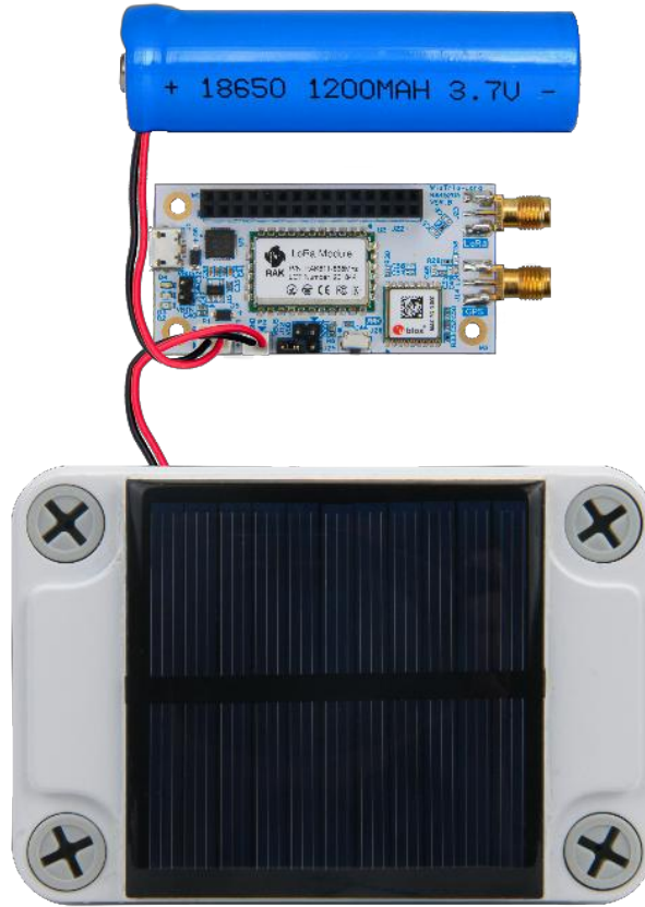
Figure 13: RAK5205 With 5V Solar Panel, Plastic Enclosure, and Li-ion Battery
