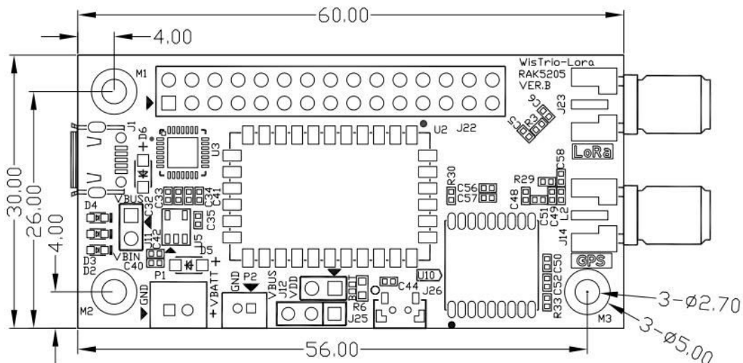
Figure 14: RAK5205 Detailed Dimensions
