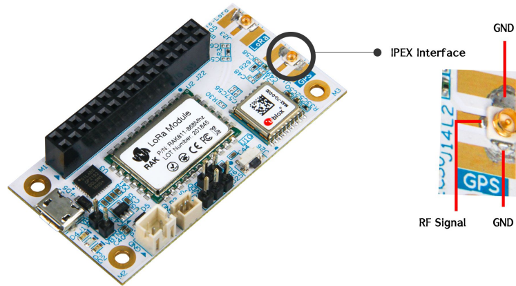
Figure 10: iPEX Interface for GPS Antenna
