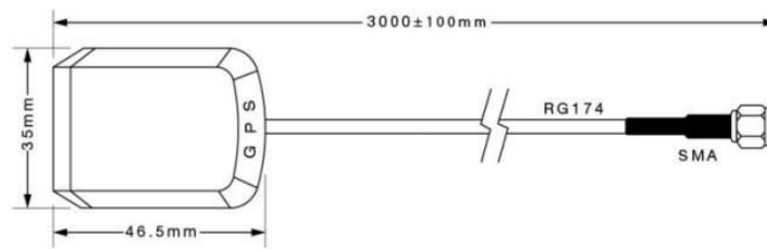
Figure 11: GPS Antenna Dimension
