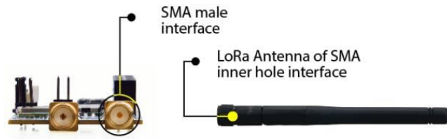
Figure 6: RP-SMA Male Connector of LoRa Antenna
