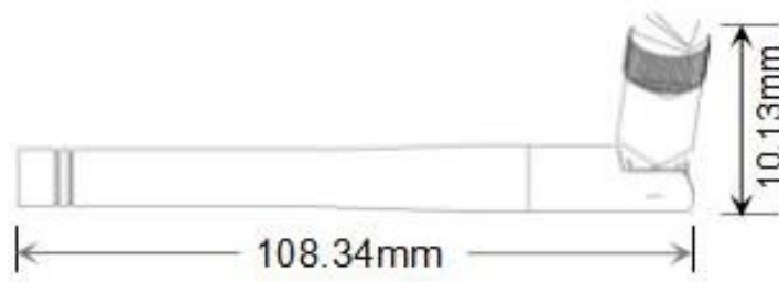
Figure 8: LoRa Antenna Dimension
