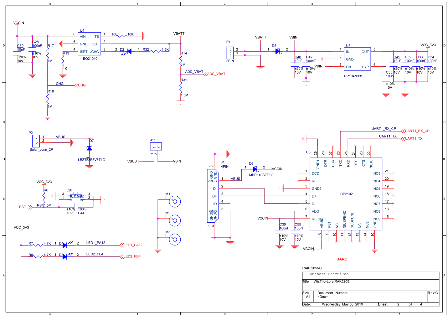
Figure 15: Schematic Diagram - 1
