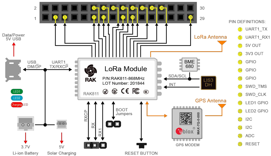
Figure 3: RAK5205 Functional Diagram
