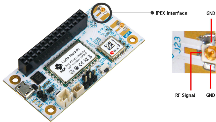
Figure 7: iPex Antenna Interface for LoRa Antenna
