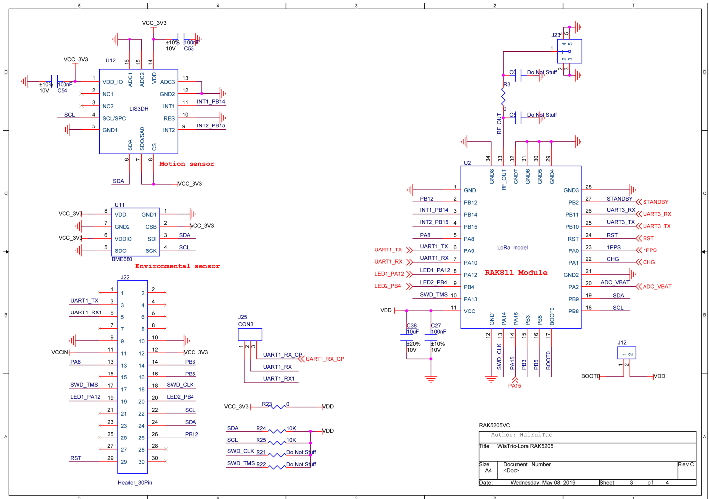
Figure 16: Schematic Diagram - 2
