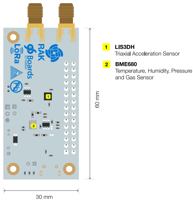
Figure 2: RAK5205 Dimension and Sensors Available
