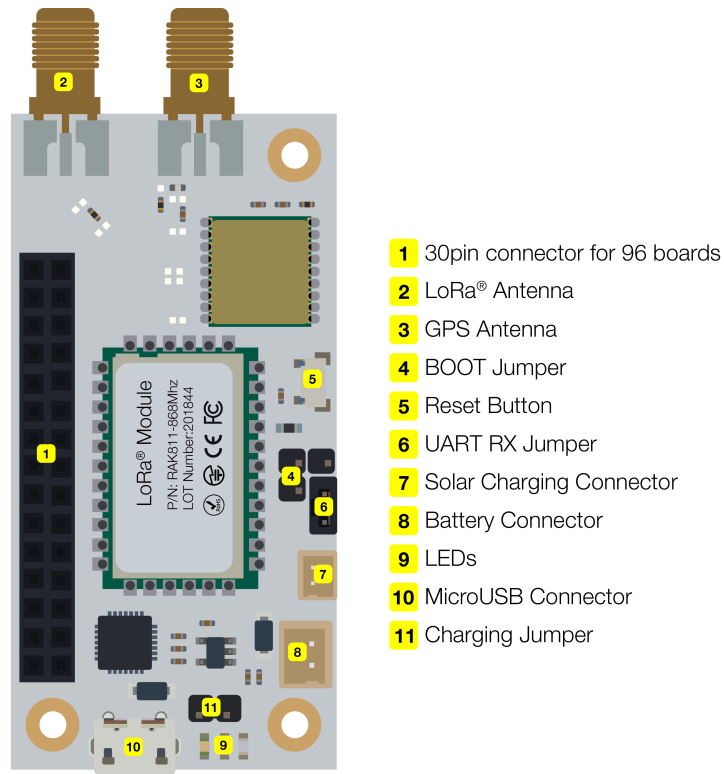
Figure 1: RAK5205 WisTrio LPWAN Tracker Interfaces
